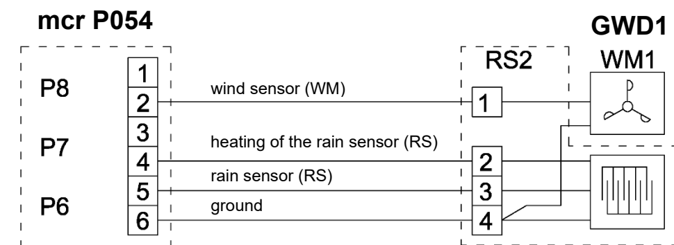
Fig. 7 Connection for the mcr P054 weather monitoring unit with a RS2-WM1 sensor and GWD-1.
